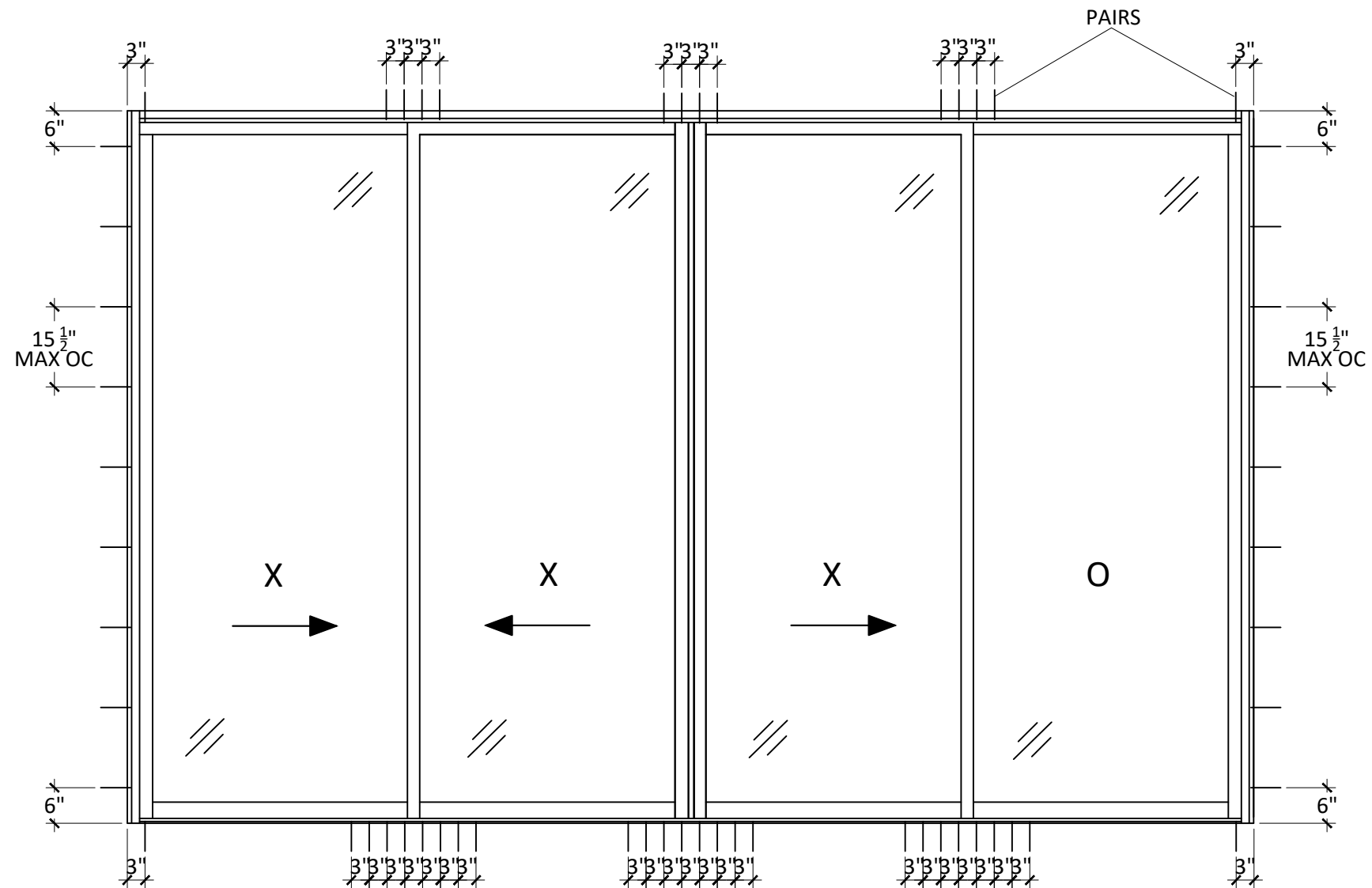
SLIDING GLASS DOOR ANCHOR LAYOUT EXTERIOR VIEW
