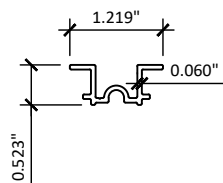
17 FIXED PANEL SUPPORT
