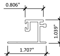
22 MONOLITHIC GLASS ADAPTER
