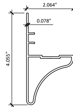
16 INTERLOCK STILE - EXTERIOR
