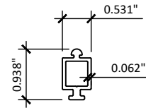
4 TRACK
