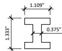
18 REINFORCING
