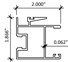
8 INTERLOCK STILE - INTERIOR
