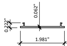
11 HEAD COVER
