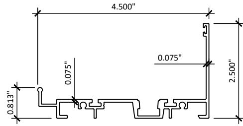
2 FRAME SILL
