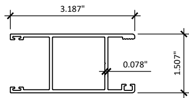
6 LOCKING STILE - FEMALE
