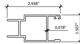
9 LOCKING STILE - MALE
