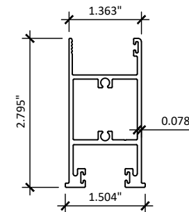
5 TOP AND BOTTOM RAIL
